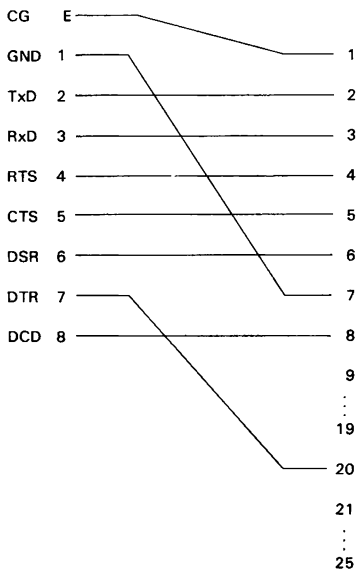
Fig. 4.15 Cable #724
